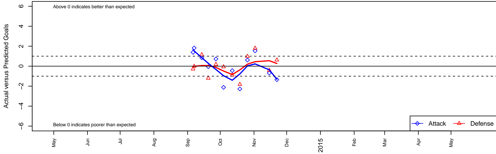
Strikers FC North McManus B95 Dots are actual minus expected GF (blue circles) and GA (red triangles). Blue line is smoothed change in attack strength. Red is smoothed change in defense strength.
